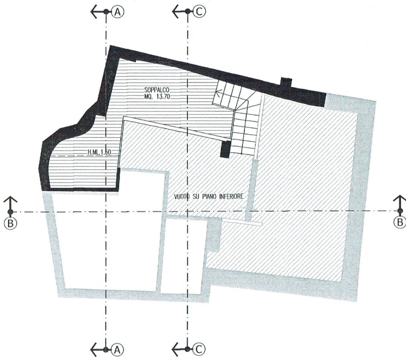
PIANTA PIANO SOPPALCO
